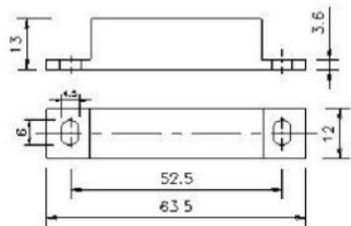
Magnet
