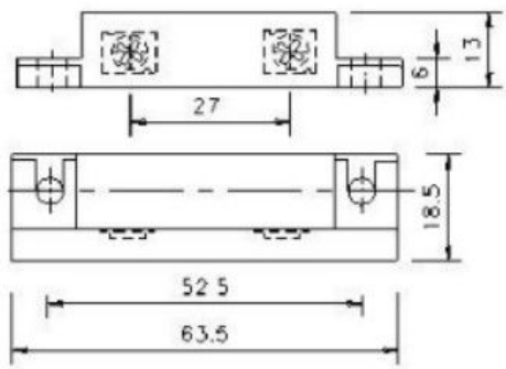
Sensor
